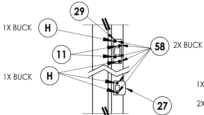
LATCH AND DEADBOLT DETAIL Kwikset Signature Series
