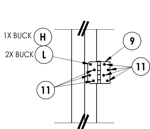
HINGE DETAIL
