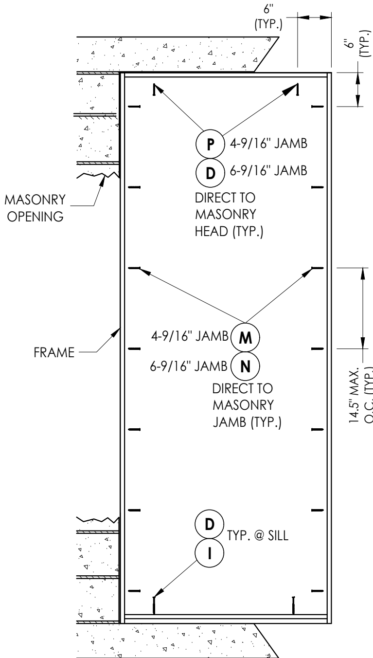
FRAME ANCHORING Direct to Masonry construction
